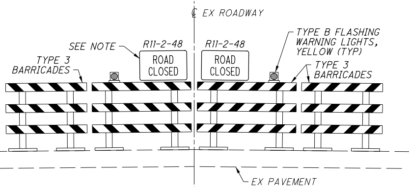
A BARRICADE CLOSURE PROFILE NOT TO SCALE FOR FURTHER INFORMATION, SEE SCD MT-101.60
